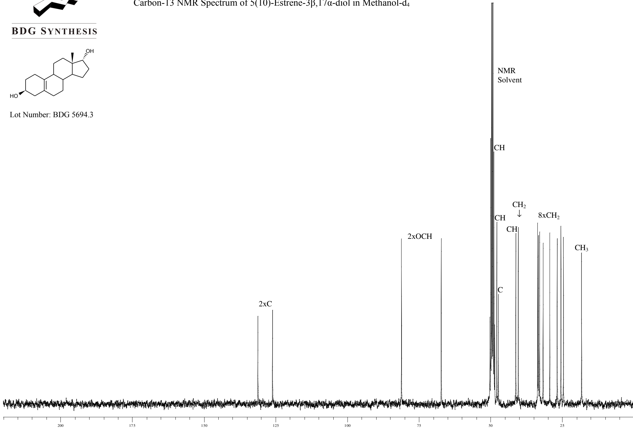
Carbon-13 NMR Spectrum of 5(10)-Estrane-3 \beta ,17 \alpha -diol in Methanol-d 4
