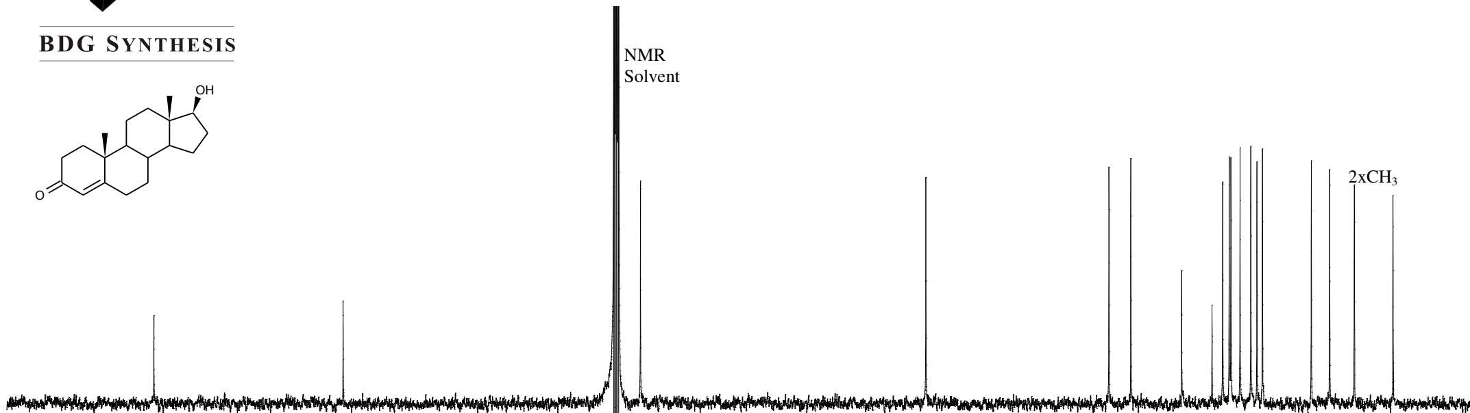
Carbon-13 NMR Spectrum of Testosterone (top) and Testosterone-19,19,19-d 3 (bottom) in C 6 D 6
